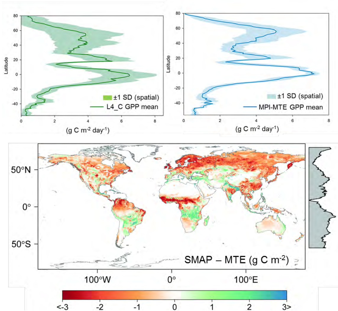
Figure 7.10. Comparison of mean daily GPP outputs (April to July; g C m -2 d -1 ) from the SMAP L4_C and MPI-MTE global data products. The L4_C outputs are derived from the initial data record for 2015, while the MTE results represent climatological means derived from a long-term (2000-2011) monthly record. The distributions of GPP spatial means and \pm 1 SD spatial variations are summarized within 0.05 degree latitudinal bins (top); the GPP difference map between the SMAP and MTE results is also shown (bottom) along with the relative mean latitudinal distribution of the GPP differences (grey shading along Y-2 axis). White areas in the difference map represent barren land, permanent ice, open water bodies and other areas outside of the L4_C product domain.
