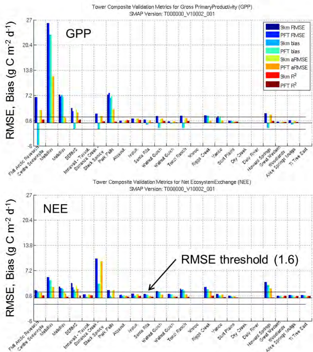
Figure 7.8. Summary of initial CVS comparisons between daily tower observations and L4_C daily product outputs for GPP and NEE from the April 15 – July 30, 2015 operational record. The reported metrics include R 2 correspondence, RMSE and bias between tower observations and L4_C spatial mean daily conditions within the overlying 9-km resolution product grid cell (9km R 2 , 9km RMSE, 9km bias); RMSE, bias and R 2 correspondence between the tower observations and the most similar PFT mean within the 9-km grid cell (PFT RMSE, PFT bias, PFT R 2 ); and the associated bias-adjusted RMSE values (aRMSE). The targeted daily NEE RMSE threshold for the L4_C product (1.6 g C m -2 d -1 ) is also shown.
