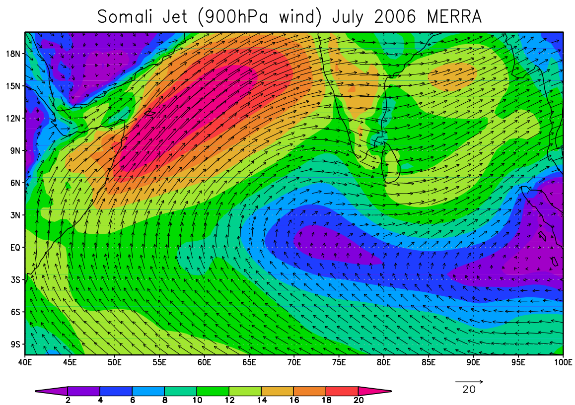
Figure 4.18: Same as Figure 4.17, but for MERRA.
