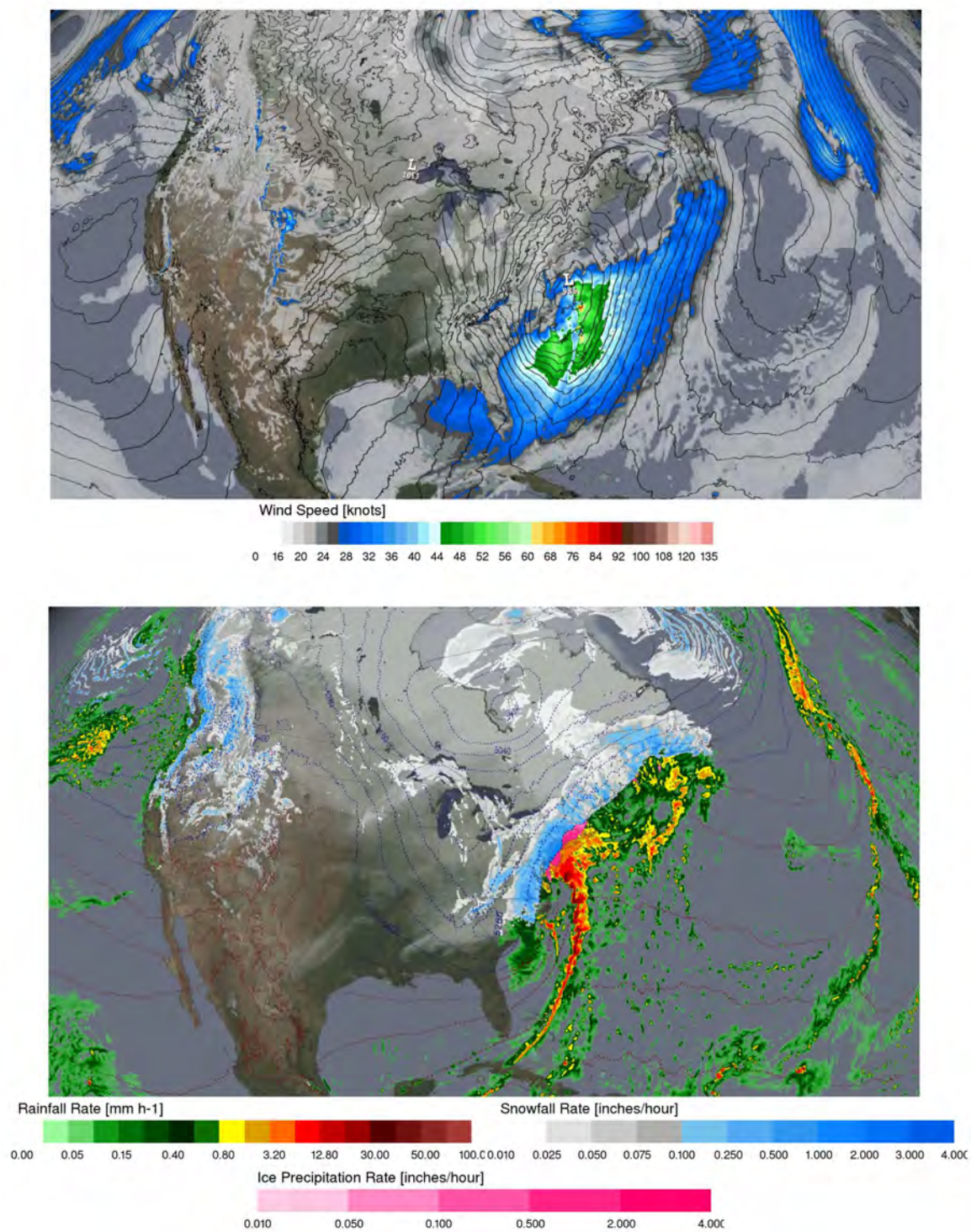
Figure 1.10: As in Figure 1.8 at 012Z January 19, 2007.
