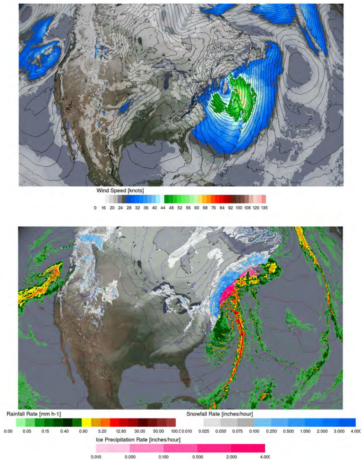
Figure 1.11: As in Figure 1.8 at 00Z January 20, 2007.
