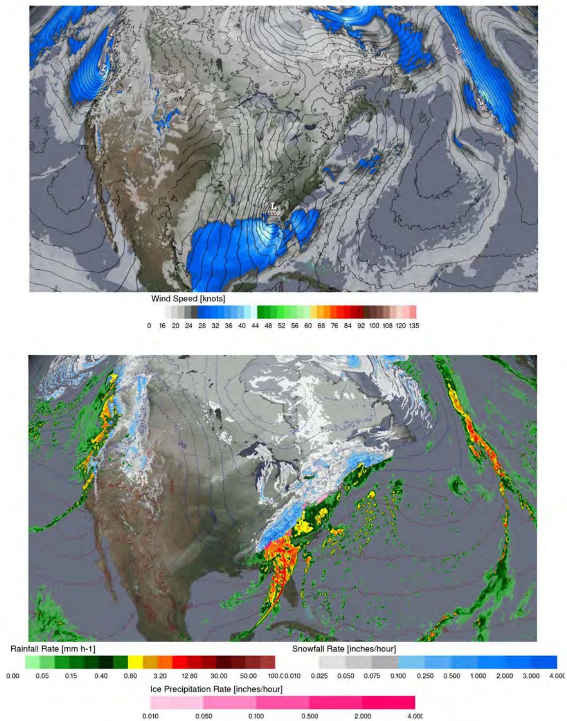
Figure 1.9: As in Figure 1.8 at 00Z January 19, 2007.
