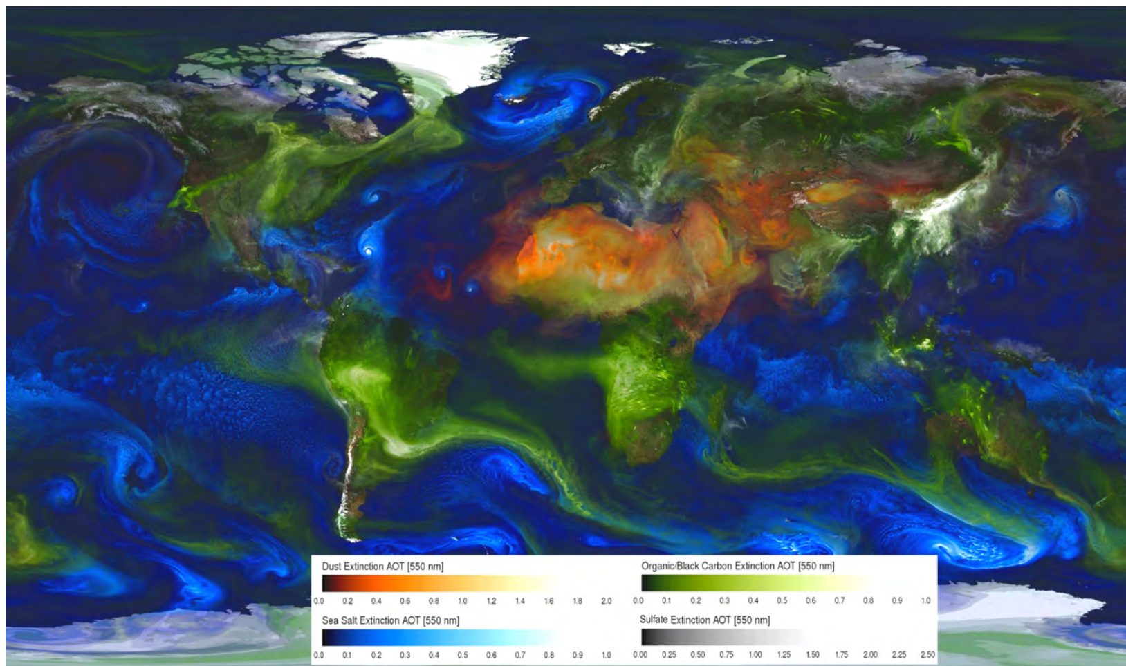
Figure 1.18: Global distribution of aerosols in the 7-km G5NR at 12Z on September 23, 2006.
