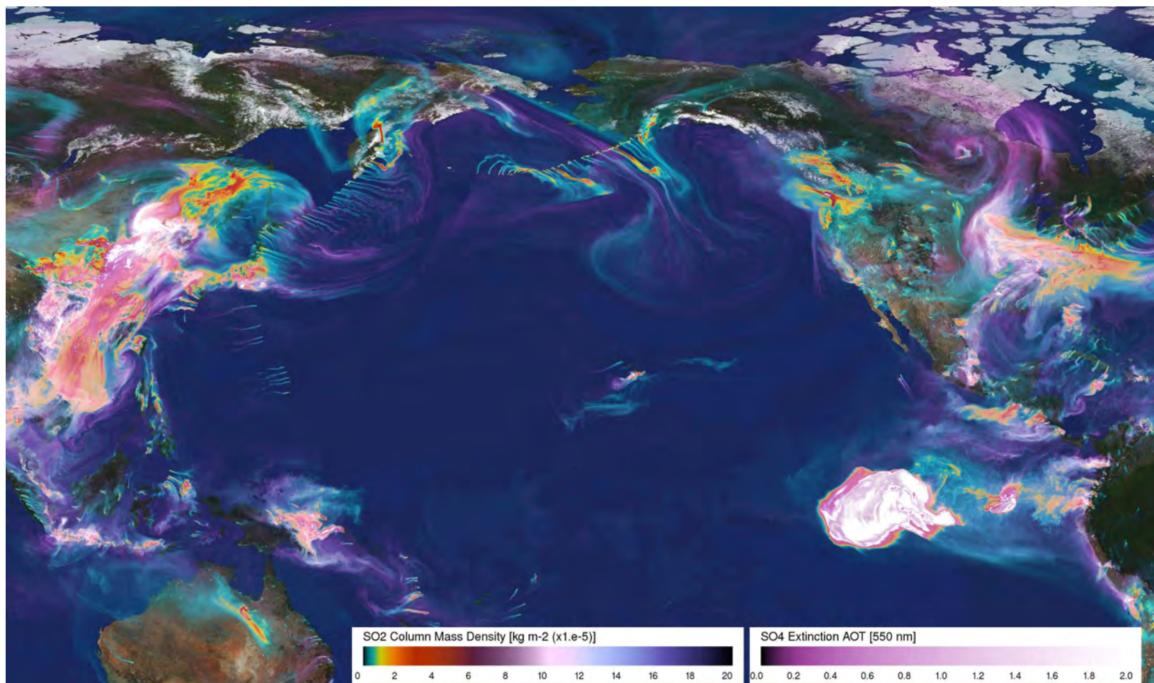
Figure 1.19: Concentrations of \text{SO}_2 and \text{SO}_4 in the 7-km G5NR at 02Z on October 27, 2005.
