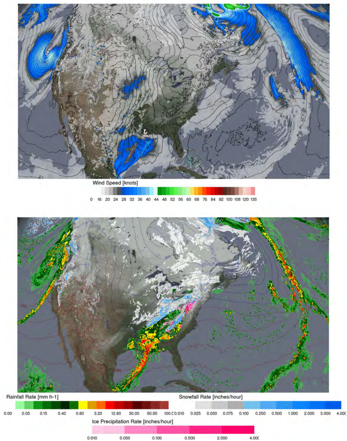
Figure 1.8: 50m-wind speeds and SLP (hPa, top), snow/ice/rain rates and 1000-500 hPa thickness contours (labeled as meters, blue \leq 5400 m, red > 5400 m, bottom) in the 7-km G5NR at 12Z January 18, 2007.
