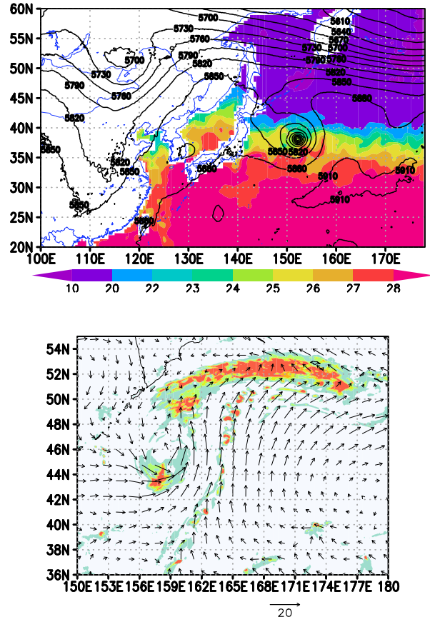
Figure 4.31: Extratropical transition of a tropical cyclone in the G5NR. Top: 500hpa geopotential height (contour, m) and sea-surface temperature (shaded, C) showing favorable positioning of tropical cyclone to upstream mid-latitude longwave trough 13 Aug. 2005, 2300 UTC. Bottom: 30-minute average rainfall rate (shaded, \text{mm d}^{-1} ) and 10m wind vectors at full ET maturity 2300 UTC 15 Aug 2005.
