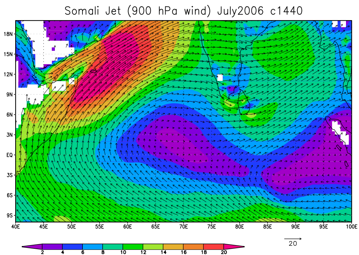
Figure 4.17: 900 hPa wind in July 2006 across the Indian Ocean in the G5NR.
