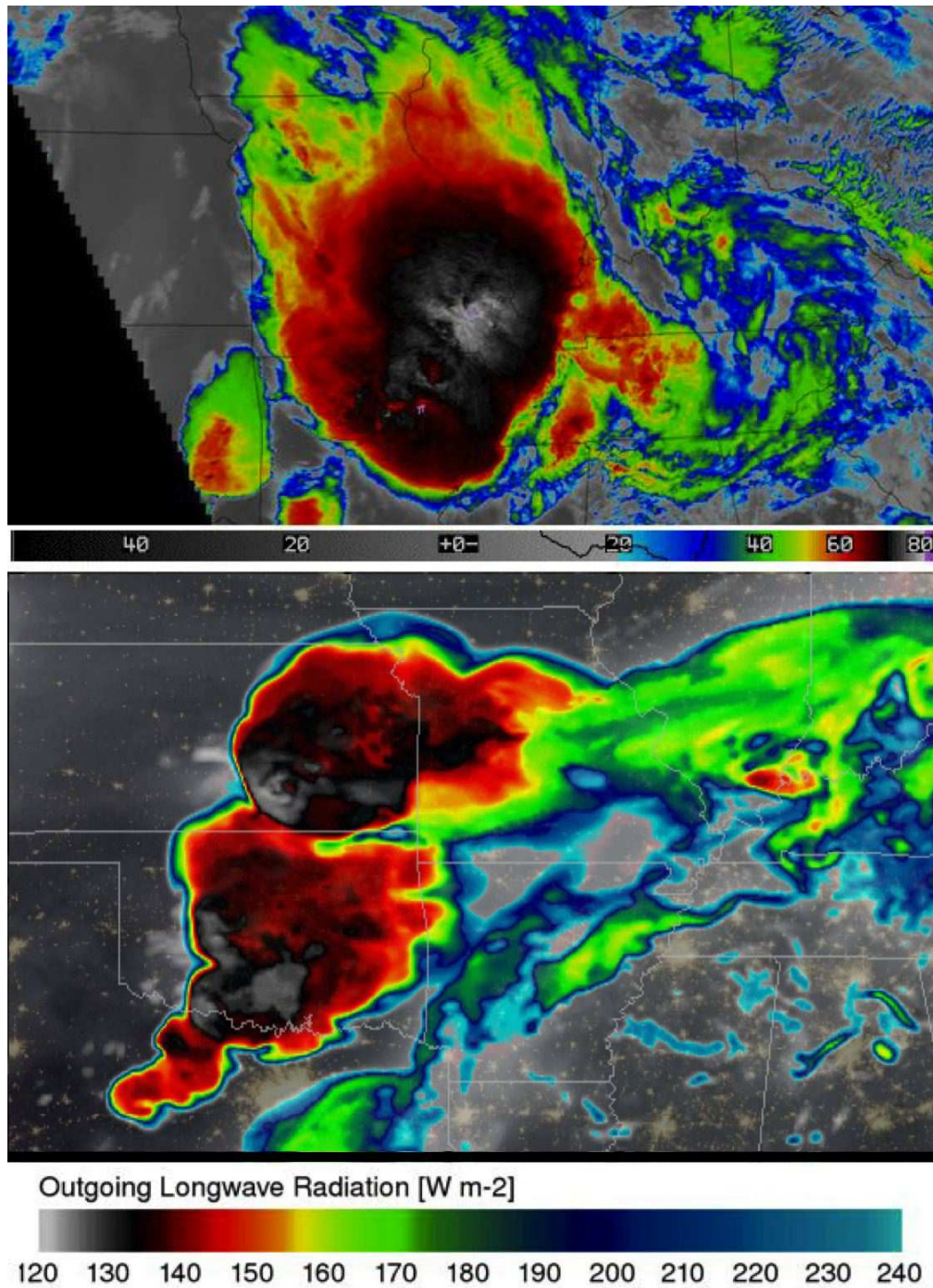
Figure 1.16: A large MCC is observed from AVHRR 15-micron IR brightness temperatures (degrees C) over the central US on April 28, 2014 at 02Z (top). A similar MCC is observed from OLR ( \text{W m}^{-2} ) in the 7-km G5NR on May 19, 2006 at 04Z (bottom).
