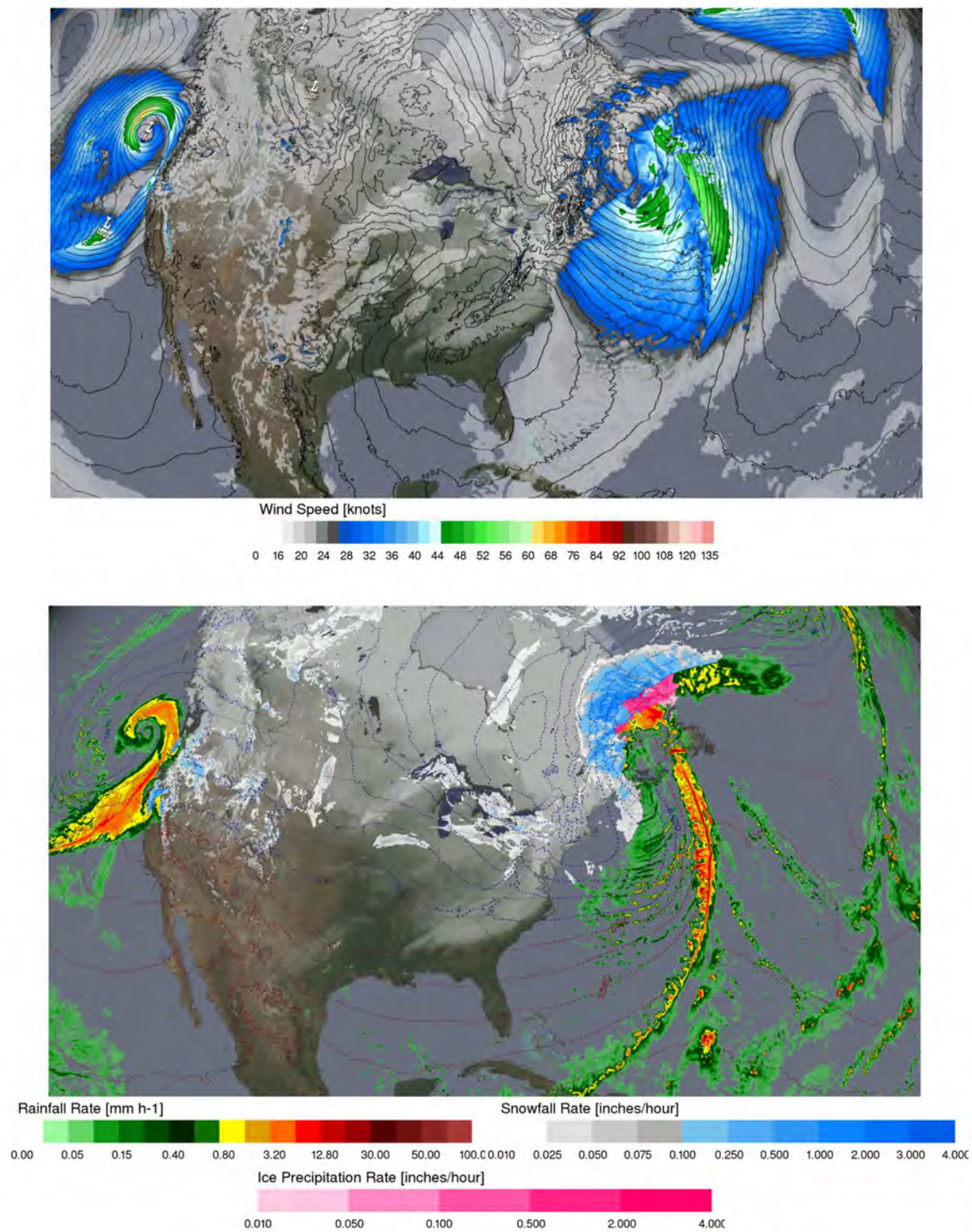
Figure 1.12: As in Figure 1.8 at 18Z January 20, 2007.
